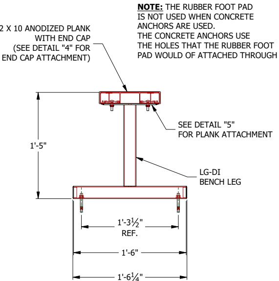
CONCRETE ANCHOR OPTION SEE DETAIL "3"
